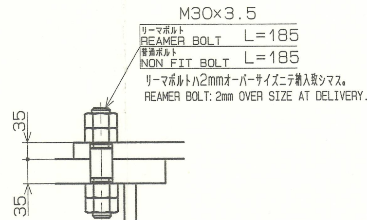
Z型推進装置据付ボルト SETTING BOLT FOR Z-TYPE PROPULSION UNIT
