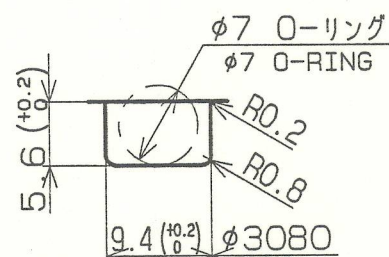
X部O-リング溝詳細 (造船所所掌) 参考 (1.5: 1) DETAIL X OF O-RING GROOVE (SHIPYARD ARRANGEMENT)
