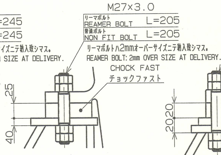
中間軸軸受据付ボルト SETTING BOLT FOR INTERM.SHAFT BEARING
